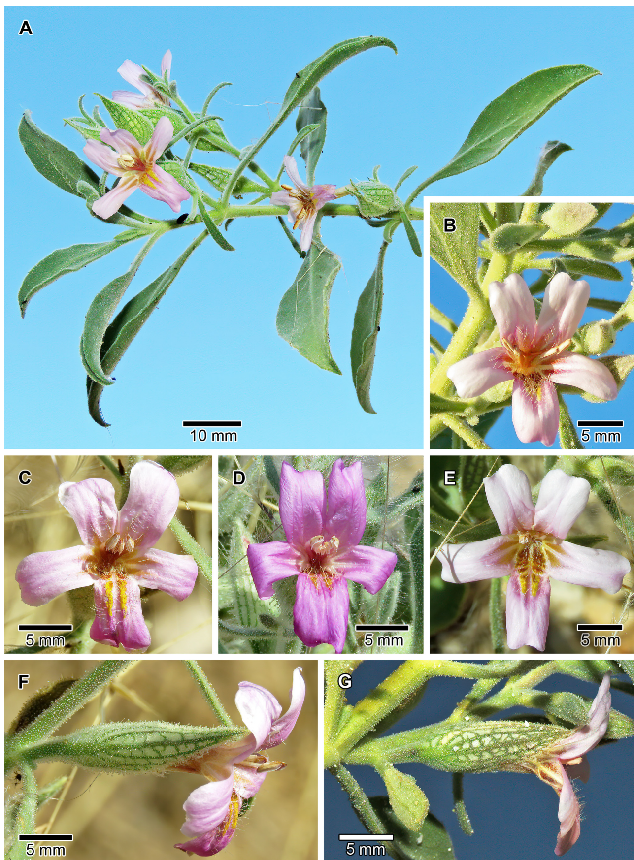
FIGURE 5. Petalidium sebrabergense . Morphology of flowers. A. Shoot with relatively narrow leaves and flowers. B, C, D, E. Flowers in front view, each from a different plant to show variation. Corolla lobes are lilac or mauve (pale violet), both surfaces concolorous. F, G. Flower in side view; bracteoles abaxially with numerous simple multi-cellular stalked glandular trichomes up to 2 mm long (not or barely visible to the naked eye), but lacking dendritic trichomes. Photographs by W. Swanepoel.
