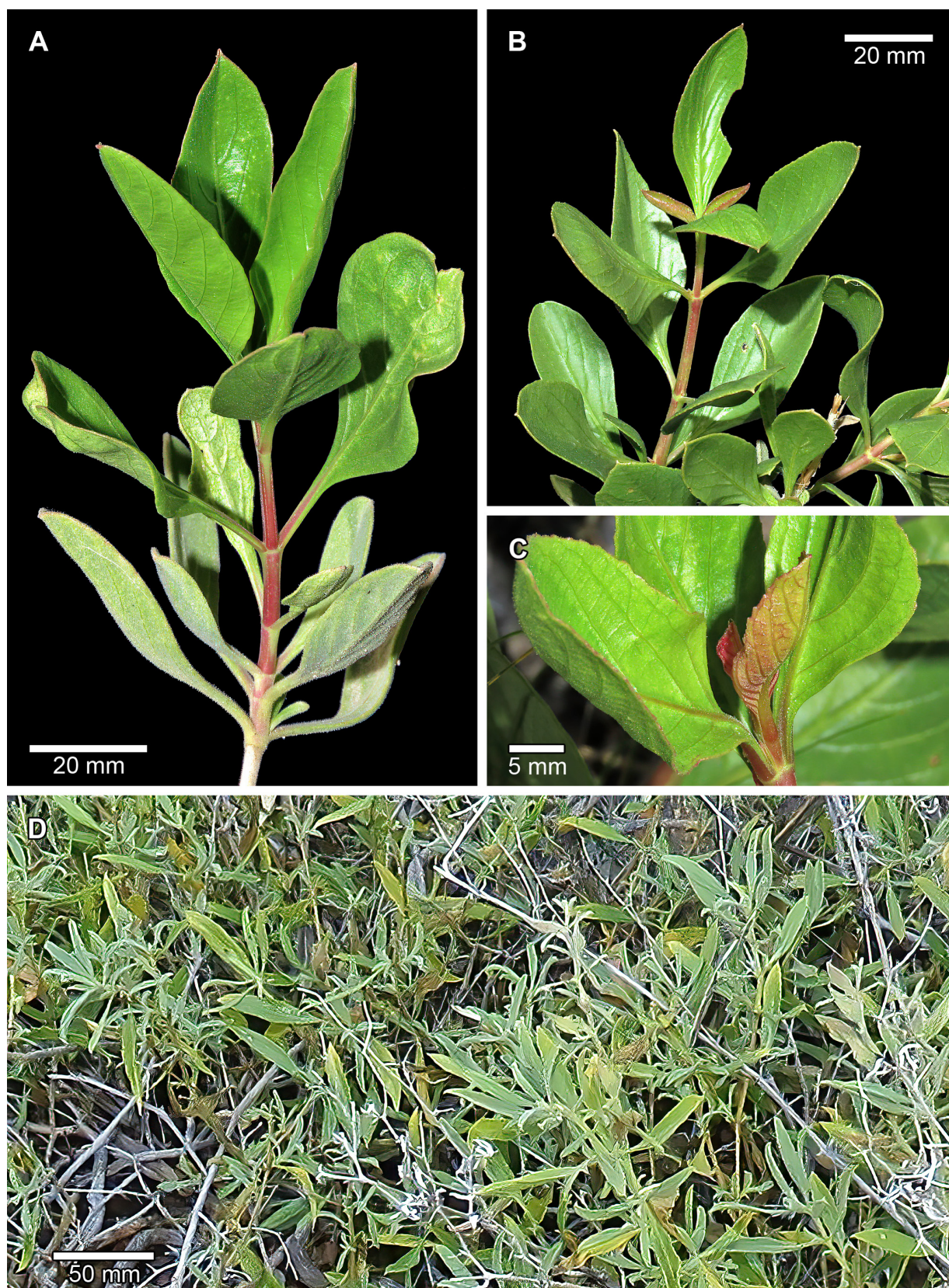
FIGURE 4. Petalidium sebrabergense . Morphology of leaves: relatively broad (A–C) and narrow-leaved forms (D). A. Shoot bearing entire-margined leaves; the older, proximal leaves have a relatively dense, but not matted, greyish indumentum likely developed under drier conditions, while the younger, distal leaves are nearly glabrous and bright green, having formed after significant rainfall. B. Shoot with leaves produced following favourable rainfall, some exhibiting denticulate or crenulate-serrate margins. C. Actively growing tip of a shoot under optimal soil moisture conditions, displaying leaves with crenulate-serrate margins. D. Leaves of narrow-leaved form. Photographs by W. Swanepoel.
