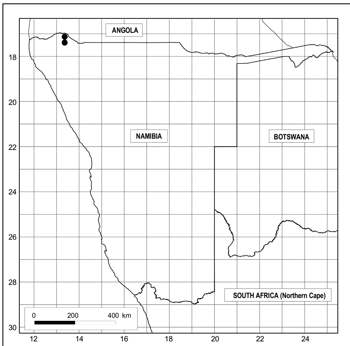
FIGURE 6. Known distribution of Petalidium sebrabergense (black dots). Based on herbarium specimens in Herb. WIND, and duplicates (still to be presented) in Herbs PRE and PRU.
