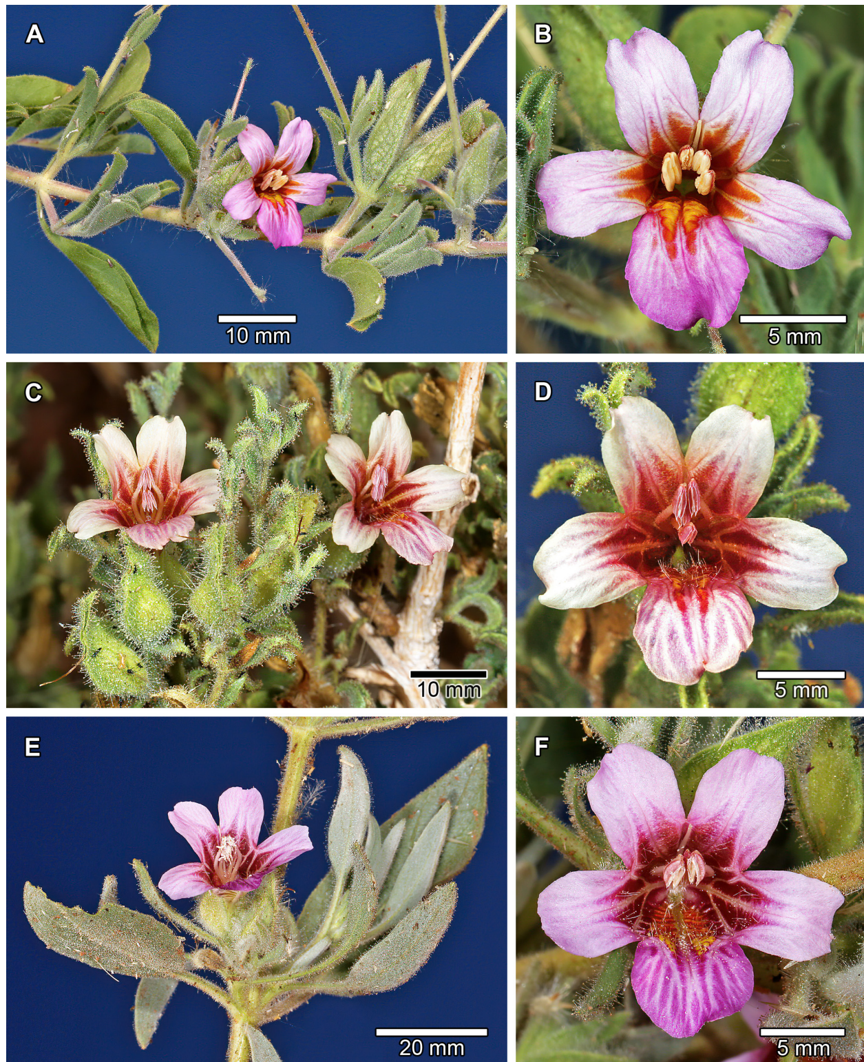
FIGURE 8. Leaf and flower morphology of three species of Petalidium with which P. sebrabergense can be confused, particularly in herbarium specimens. A, B. P. huillense , branchlet with leaves and flowers (A); flower in front view (B). C, D. P. subcrispum , branchlet with leaves, flowers and persistent bracteoles of spent flowers (C); flower in front view (D). E, F. P. welwitschii , branchlet with leaves and flower (E); flower in front view (F). Photographs by W. Swanepoel.
