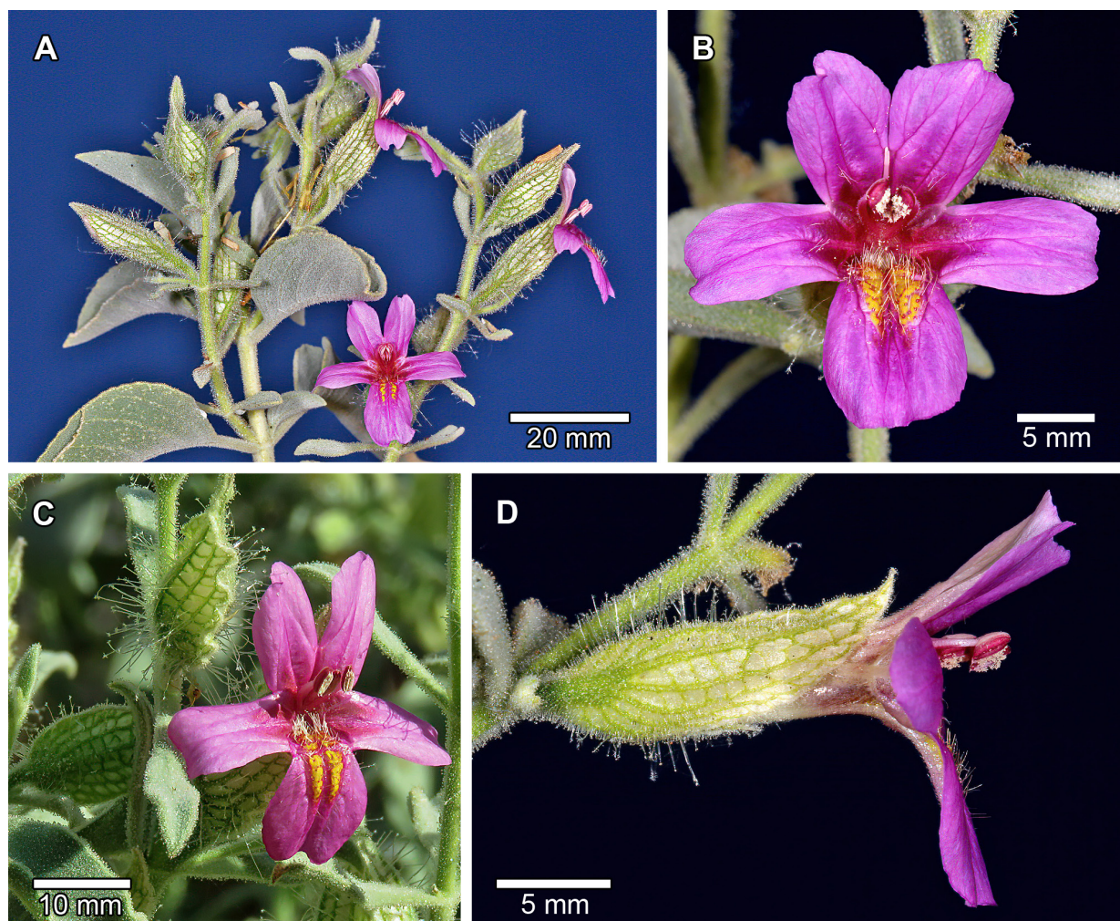
FIGURE 7. Petalidium cirrhiferum . Morphology of leaves and flowers. A. Branchlet showing ovate or narrowly ovate leaves with greyish indumentum composed of matted dendritic and bifurcate trichomes (microscopic enlargement required). B. Flower in front view. C. Flower in front view and persistent bracteoles of spent flowers. Note outer surface of bracteoles with robust, long-stalked dendritic trichomes up to 5 mm long. D. Flower in side view, showing bracteole with long-stalked dendritic trichomes. Photographs by W. Swanepoel.
