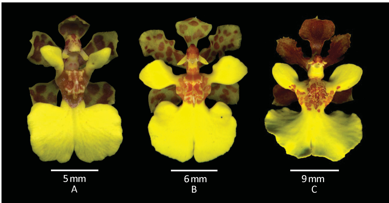
FIGURE 5. Morphological comparison of Cohniella ×francoi and putative parents. A. Cohniella ascendens (Costa Rica, based on Pupulin 5784, JBL). B. Cohniella ×francoi (Costa Rica, Pupulin s.n. sub Carnevali 7257, CICY). C. Cohniella brachyphylla (Costa Rica, Bogarin 6153, JBL).
