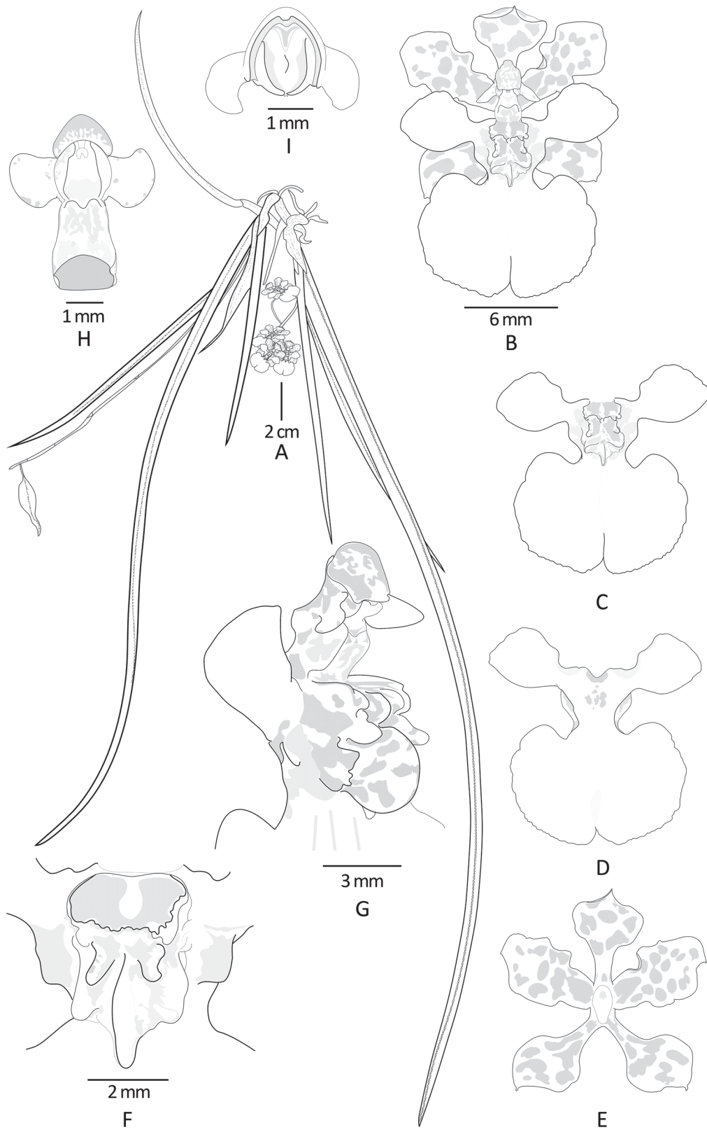
FIGURE 1. Cohniella × francoi . A. Habit with inflorescence. B. Flower. C. Labellum front view. D. Labellum back view. E. Sepals and petals. F. Disc and callus. G. Column and base of labellum, lateral view. H. Column, ventral view. I. Column, front view. Scale: B-E. 6 mm. Drawing by W. Cetzal-Ix.
