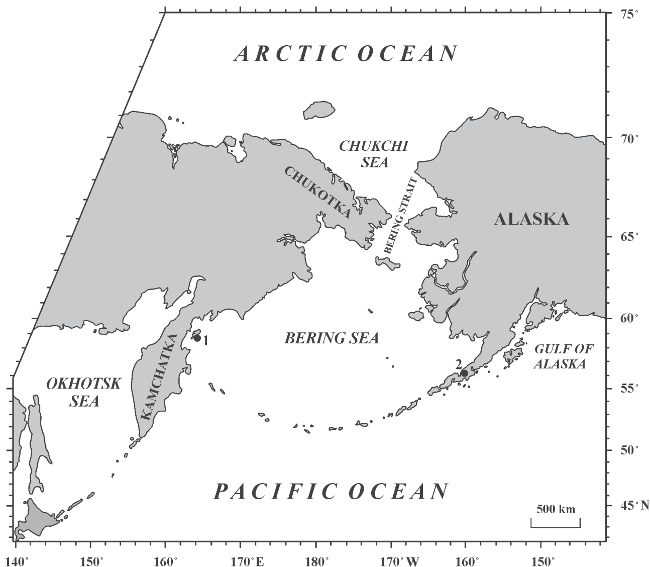
FIGURE 1: Locations of the Cenozoic stratigraphic sections (black circles) in the North Pacific region where Thalassiosira dolmatovae is documented. 1—Karaginsky Island section, northeastern Kamchatka. 2—Sandy Ridge section, the Alaska Peninsula, southwestern Alaska
