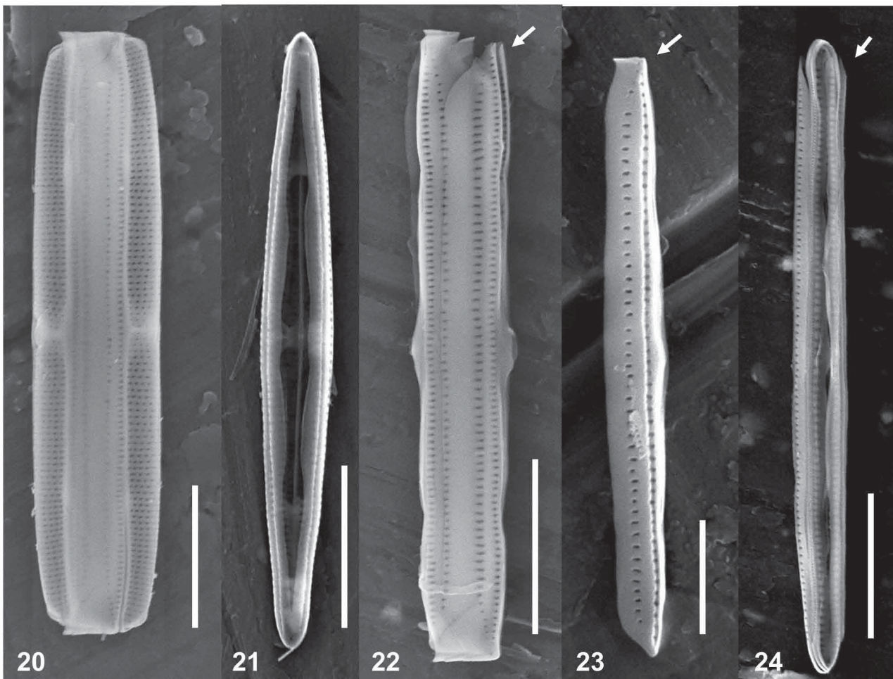
FIGURES 20–24. Tursiocola ziemanii . Type population, SEM. 20. Entire frustule in girder view showing cingulum with 2 copulae, each with a double row of pores. 21. Internal view of valve with attached copula. 22. Cingulum comprised of 2 copulae open on one end (arrow) with 2 rows of pores. 23. Isolated copula showing closed end (arrow) and two rows of pores. 24. Internal view of cingulum showing open (arrow) and closed ends of copulae. Scale bars: 20–22, 24 = 10 \mu\text{m} ; 23 = 5 \mu\text{m} .
