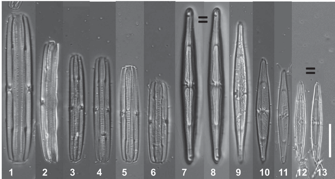
FIGURES 1–13. Tursiocola ziemanii . Type population, LM. 1–6. Frustules in girdle view showing size range and morphological variation. 7–13. Specimens in valve view showing size range. Scale bars: 1–13 = 10 \mu\text{m} . = indicates same specimen at different foci.
