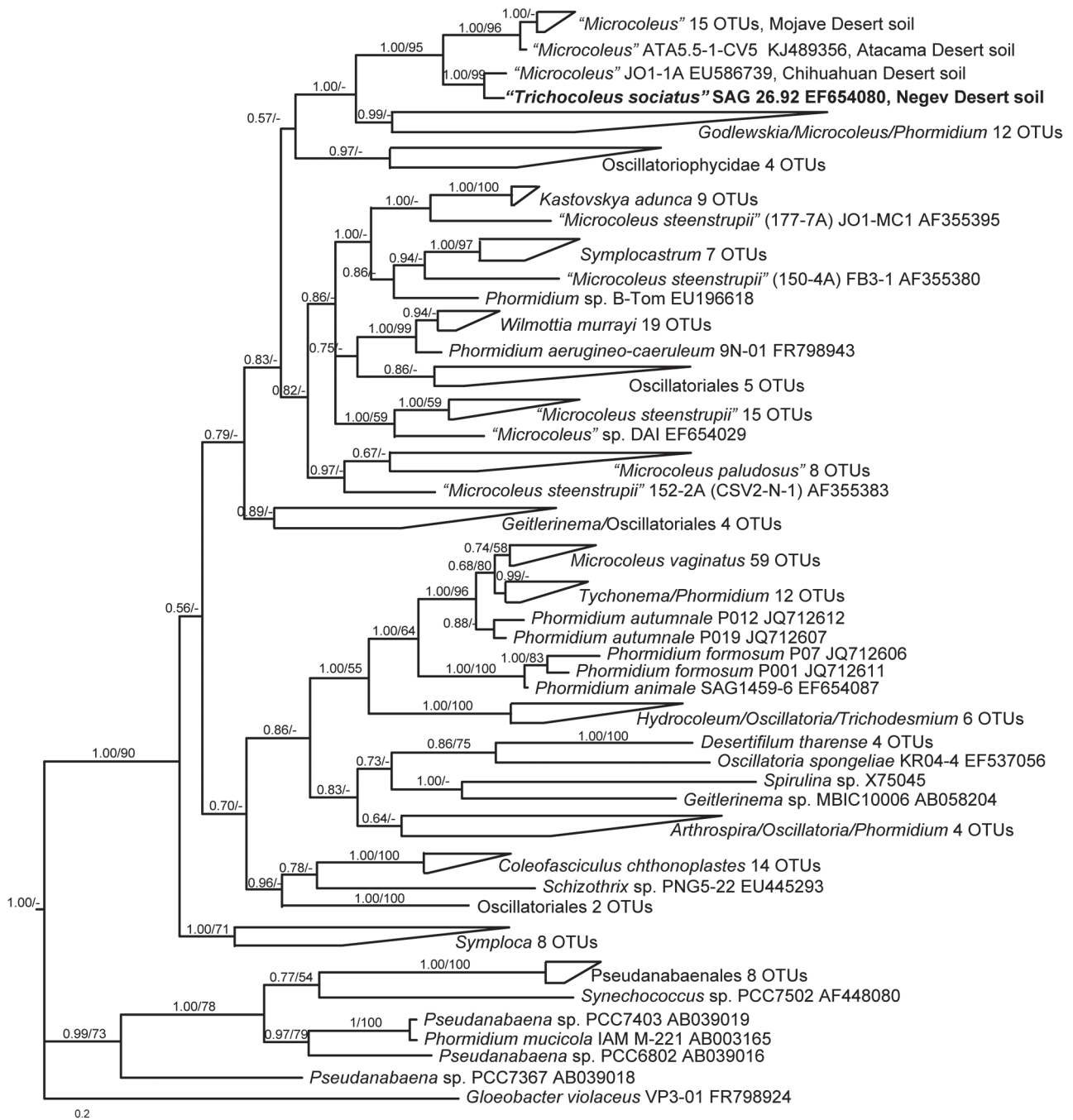
FIGURE 10. Bayesian analysis of 225 strains within the Oscillatoriales showing the phylogenetic position of Trichocoleus (Microcoleus) sociatus SAG 26.92 in a clade of an unnamed desert soil genus outside of the Microcoleus sensu stricto . Taxonomic epithets applied to GenBank sequences that we consider to be incorrect are indicated by enclosure in quotation marks.
