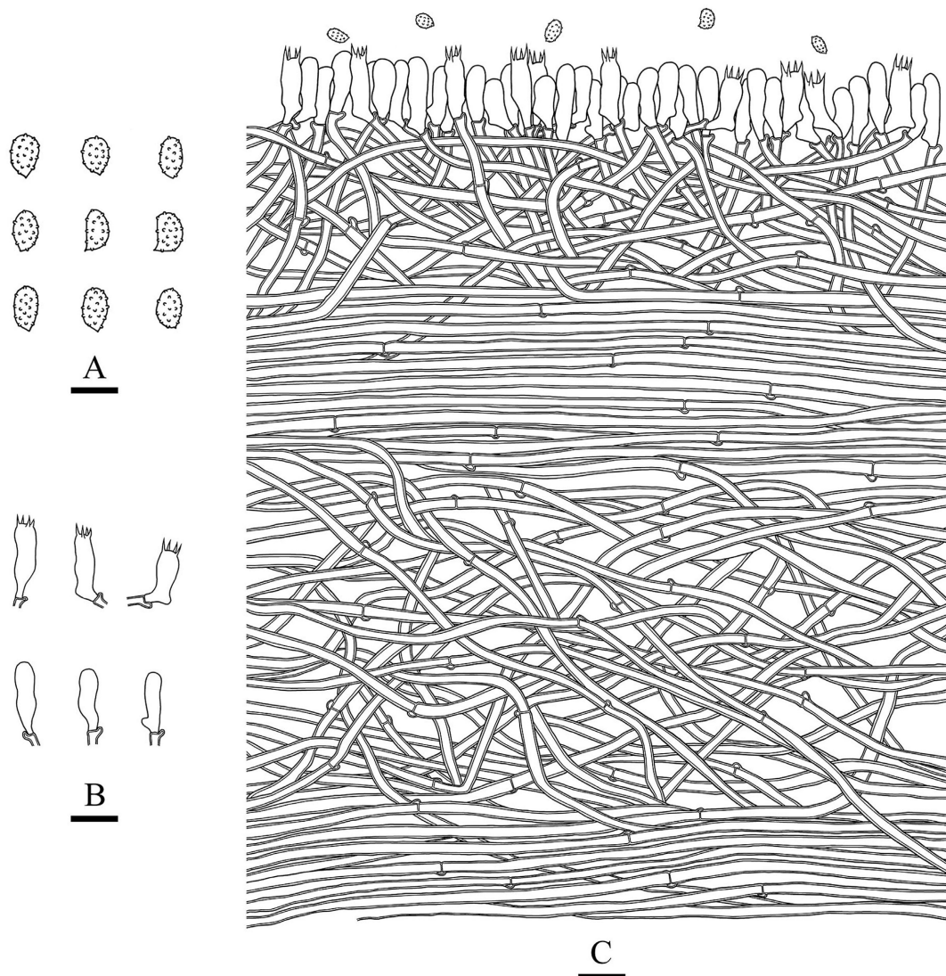
FIGURE 4. Microscopic structures of Xenasmattella rhizomorpha (drawn from the holotype). A. Basidiospores. B. Basidia and basidioles. C. A section of hymenium. Bars: A = 5 µm; B, C = 10 µm.
