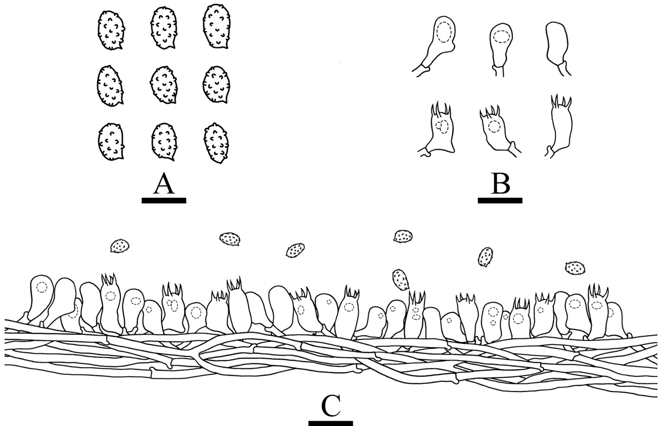
FIGURE 5. Microscopic structures of Xenasmatella tenuis (drawn from the holotype). A. Basidiospores. B. Basidia and basidioles. C. A section of hymenium. Bars: A = 5 \mu\text{m} ; B, C = 10 \mu\text{m} .
