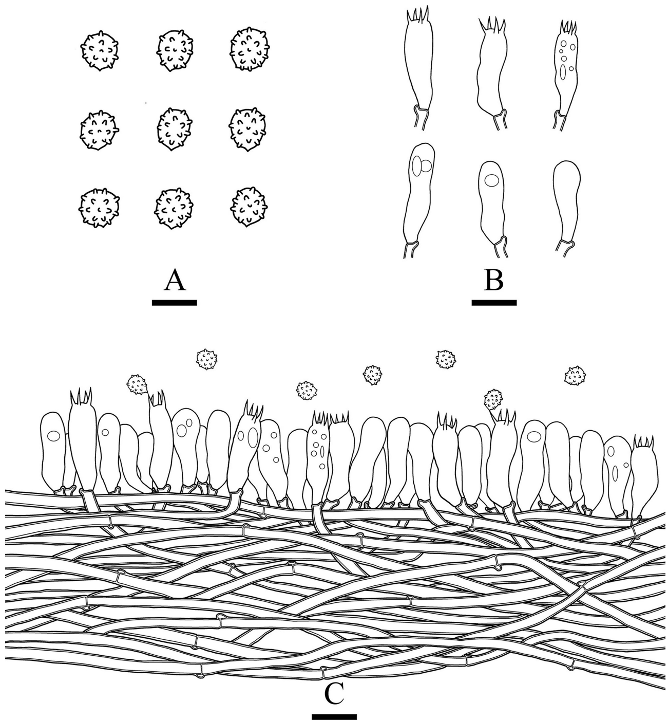
FIGURE 6. Microscopic structures of Xenasmatella xinpingensis (drawn from the holotype). A. Basidiospores. B. Basidia and basidioles. C. A section of hymenium. Bars: A = 5 \mu\text{m} ; B, C = 10 \mu\text{m} .
