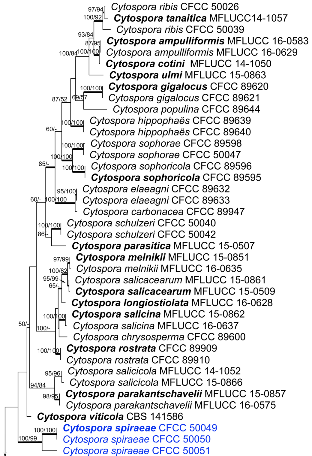
FIGURE 2. Phylogram of Cytospora based on combined ITS, LSU, ACT and RPB2 genes. MP and ML bootstrap support values above 50 % are shown at the first and second position. Thickened branches represent posterior probabilities above 0.95 from BI. Ex-type strains are in bold. Strains in current study are in blue.
