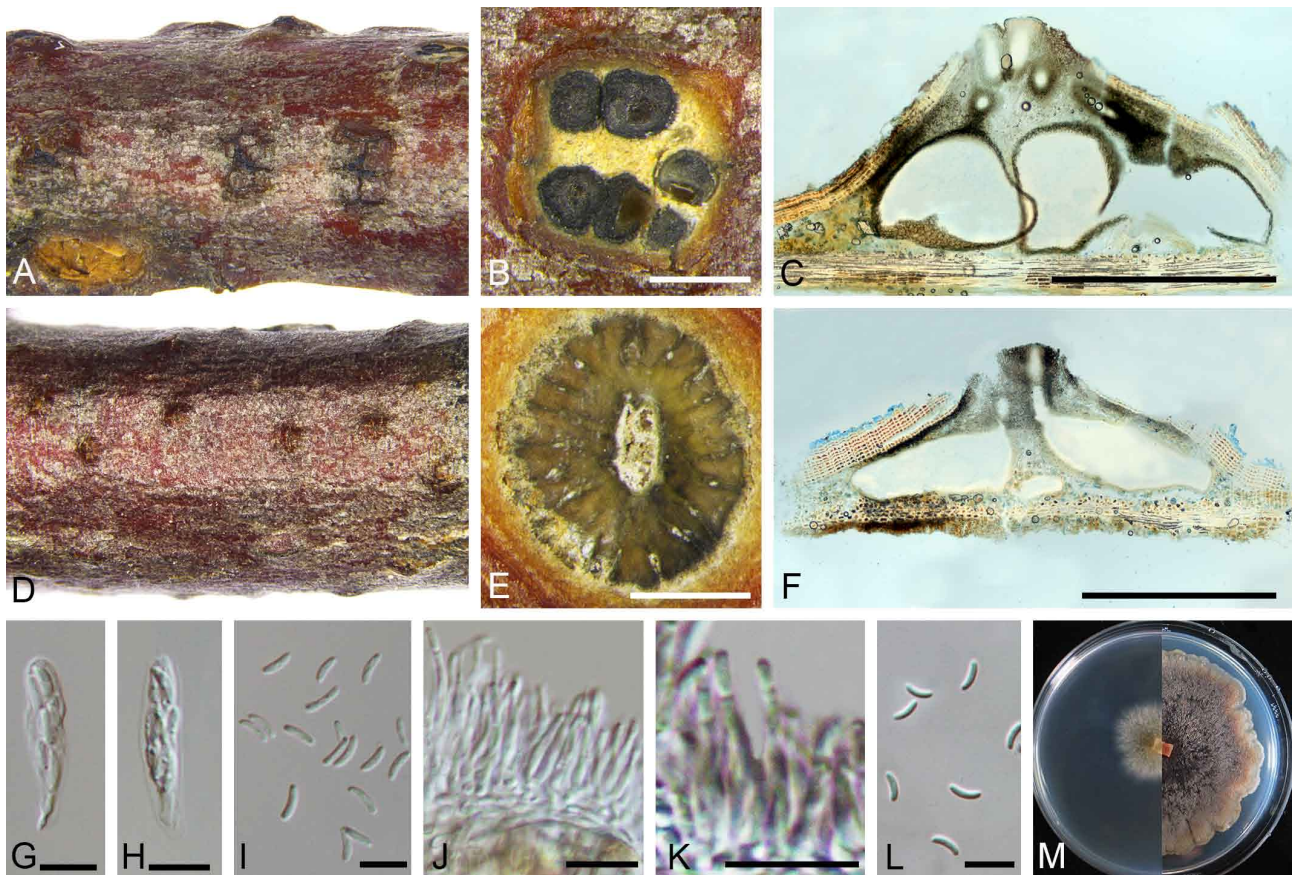
FIGURE 3. Morphology of Cytospora spiraeae from Spiraea salicifolia (BJFC-S784). A: Habit of ascomata on twig. B: Transverse section of ascomata. C: Longitudinal section through ascomata. D: Habit of conidiomata on twig. E: Transverse section of conidiomata. F: Longitudinal section through conidiomata. G–H: Asci. I: Ascospores. J–K: Conidiophores and Conidiogenous cells. L: Conidia. M: Colonies on PDA at 3 days (left) and 30 days (right). Scale bars: B–C, E–F = 500 \mu m; G–L = 10 \mu m.
