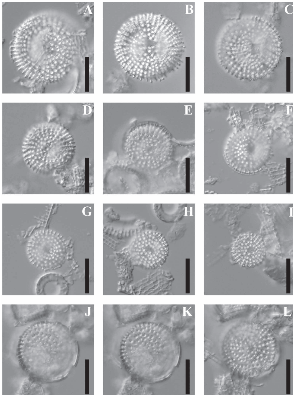
FIGURE 7. Diminution size series of L. cohenii (A–I). The Holotype at differing focal planes (J–L).
