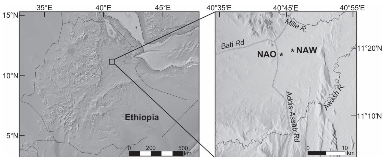
FIGURE 1. Location of the NAO and NAW drill core sites in the Afar Depression of Ethiopia.
