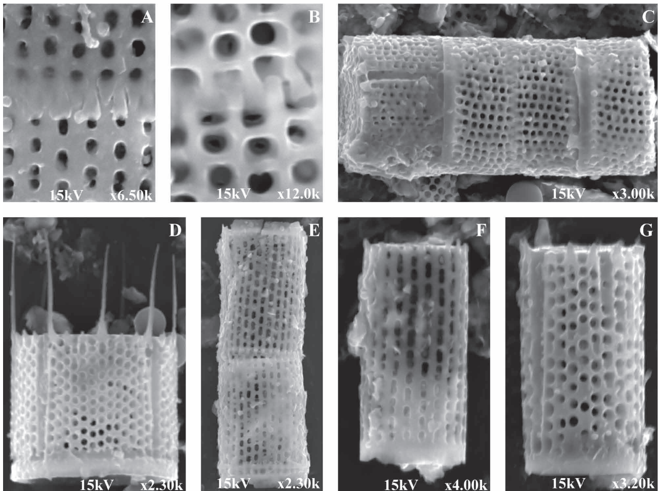
FIGURE 6. Scanning electron micrographs of A. jewsonii . Spatulate linking spines of two internal sister valves (A). Note the doubly punctate areolae that is typical of internal valves (E). Spatulate linking spines are also present on linking valves (B) that sometimes exhibit twisting costae (C). A filament of two frustules, one contains a separation valve (C) (far left), and a linking valve (middle left), the frustules on right contains two linking valves. A well preserved separation valve (D). Sister internal valves held together by spatulate linking spines (E). A single internal valve (F). A single separation valve (G).
