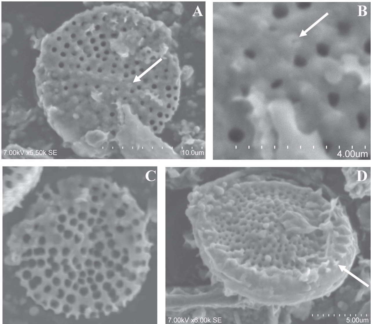
FIGURE 8. Scanning electron micrographs of L. cohenii . Central fultoportula arrowed (A, B). A heavily dissolved specimen (C). Isometric view of a well preserved specimen exhibiting transverse undulation, spinules arrowed (D).
