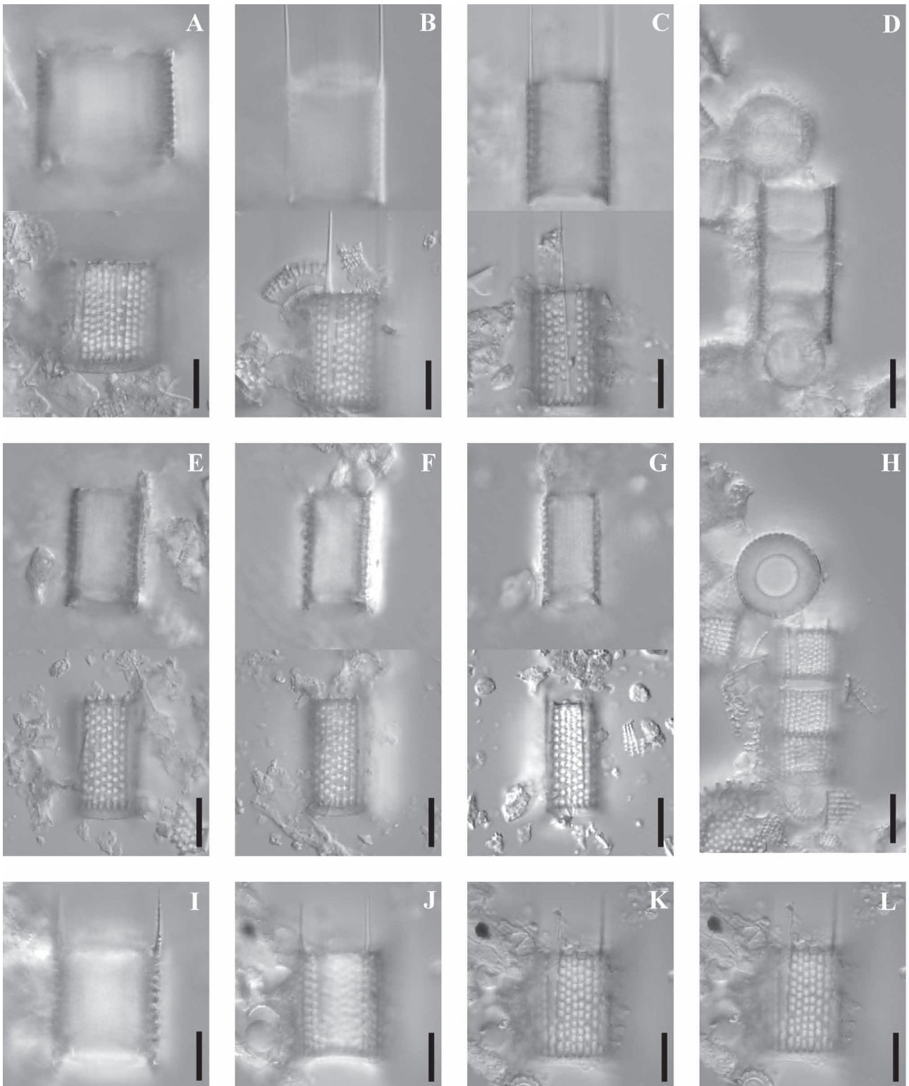
FIGURE 5. Diminution size reduction series pictures of A. jewsonii taken at two focal heights to examine the diameter accurately (A–C, E–G). Three valves in a filament (D, H) the top valve is a separation valve while the bottom two are linking valves. The holotype is shown at different focal heights (I–L).
