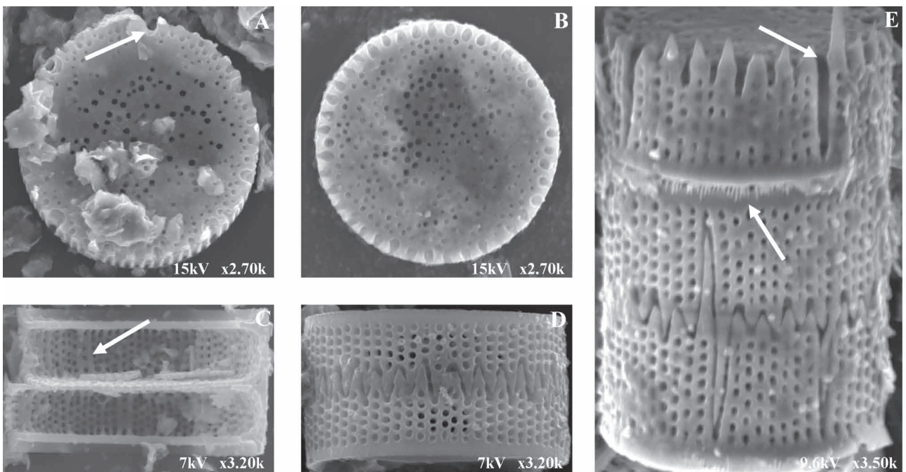
FIGURE 4. Scanning electron micrographs of A. helianthus . (A) Valve view of a separation valve. Note the separation furrow (arrowed). A linking valve (B) in valve view lacks separation spines and furrows. Internal view of two separation valves (C) two thickened costae are the internal structure of the separation furrow (arrowed). Two linking valves lacking separation spines (D). A filament of A. helianthus with separation furrow arrowed (E). Fimbriae attach the two valves of the frustule (E), arrowed.
