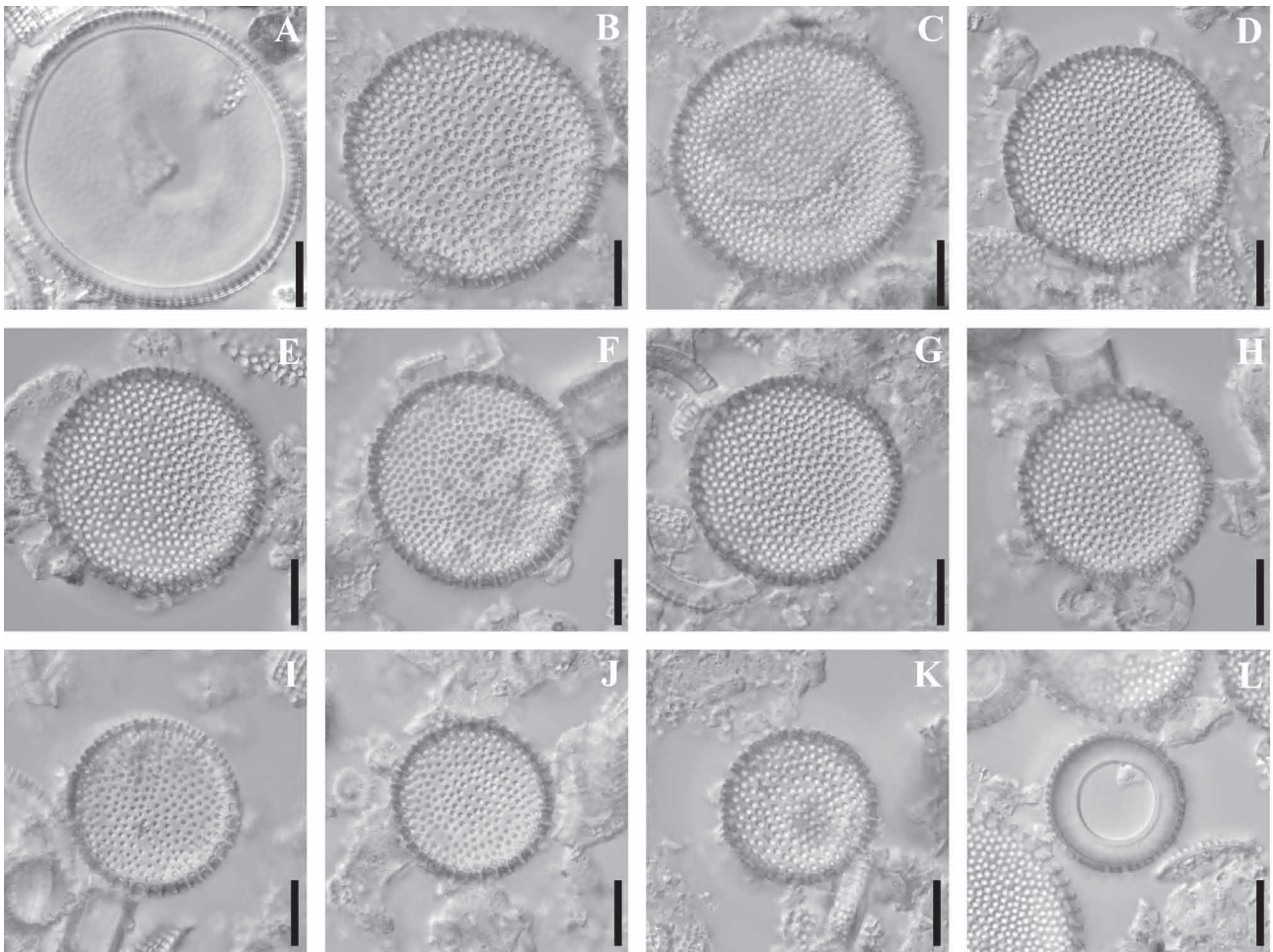
FIGURE 3. Size diminution series of A. helianthus (A–L). Holotype shown (B). Ringleiste view (A, L). Scale bars are 10 µm throughout.
