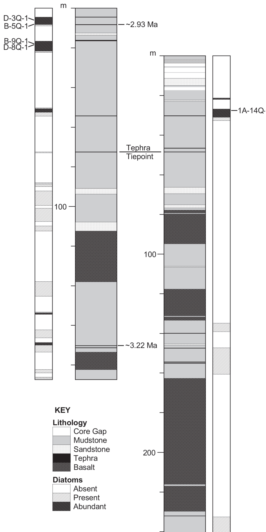
FIGURE 2. Simplified lithology of the NAO and NAW drill cores. NAO14-1B/1D is a composite of NAO14-1B with gaps filled in by NAO14-1D. A tephrostratigraphic tie point correlates NAO with NAW at ~75 mbs and ~50 mbs, respectively. Diatom presence from initial 32 cm sampling
