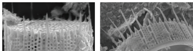
FIGURE 9. Scanning electron micrographs of Aulacoseira helianthus (left) and A. agassizii var. malayensis (right). Note the spine morphology originating from two mantle costae, location of the separation furrow in relation to the separation spine, and spine distribution.
