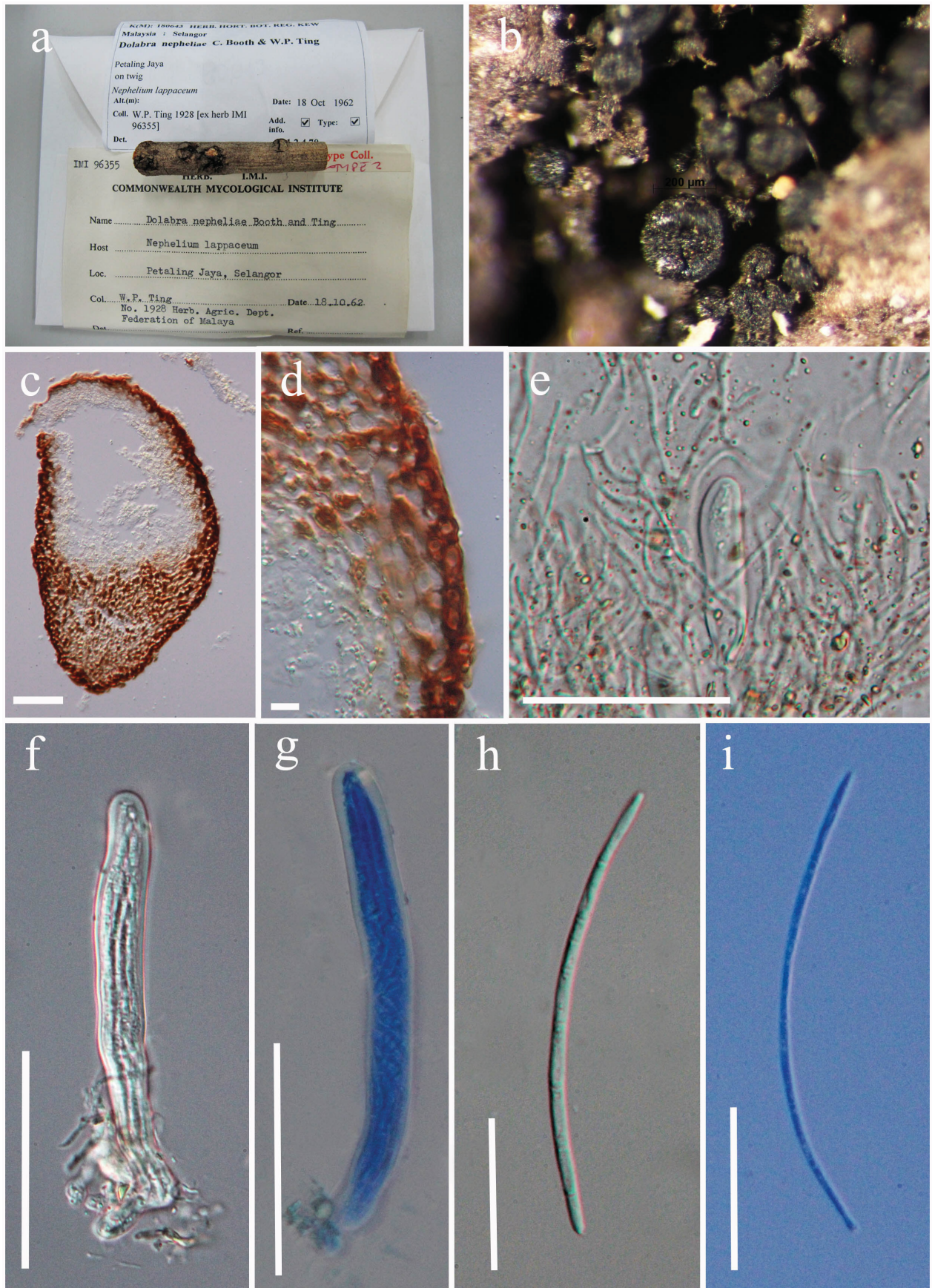
FIGURE 5. Dolabra nepheliae (holotype). a. Herbarium material. b. Ascomata on host surface. c. Section of an ascoma. d. Section of the peridium. e. Pseudoparaphyses. f–g. Asci (blue staining in lactophenol cotton blue reagent). h–i. Septate, long, cylindrical ascospores. Scale bars: c = 50 µm, d = 10µm, e–g = 50 µm, h–i = 25 µm.
