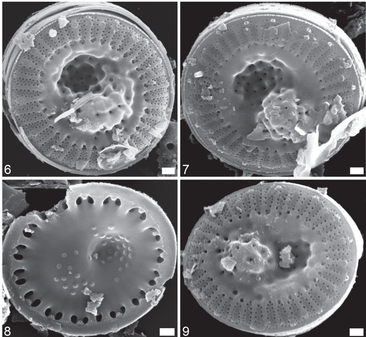
FIGURES 6–9: Cyclotella idahica . SEM. Figures 6, 7, 9, external views. Valve views showing transversely undulate central area with irregularly arranged areolae and covered by bumps. Present are external openings of areolae and short tubes of marginal fultoportulae. Spines and/or spines bases are found on the valve face/mantle junction. Scale bars = 1 \mu\text{m} . Figure 8, internal view. Valve view showing location of one fultoportula on the valve face. Arrow indicates position of the rimoportula. Scale bar = 1 \mu\text{m} .
