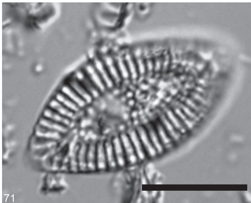
FIGURES 70–71: Cyclotella jonesii . LM. Figure 70 is of Morphotype 1. Figure 71 is of Morphotype 2. Scale bars = 10 \mu m.
